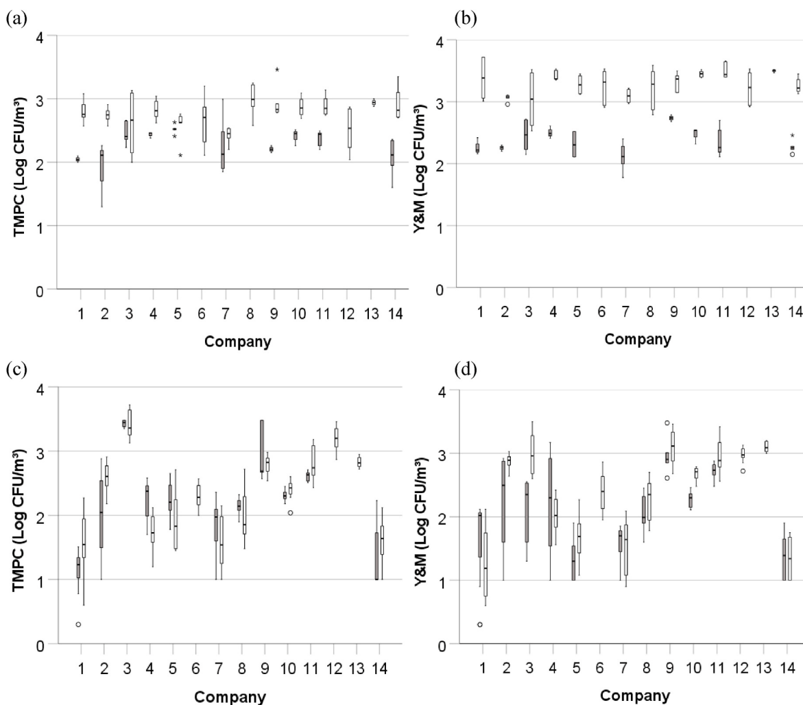
Fig. 3. Comparison of outdoor total mesophilic plate count (TMPC) (a), yeast and mould (Y&M) count (b) and indoor TMPC (c), Y&M (d) (log cfu/m 3 ), in winter ■ and summer □.
