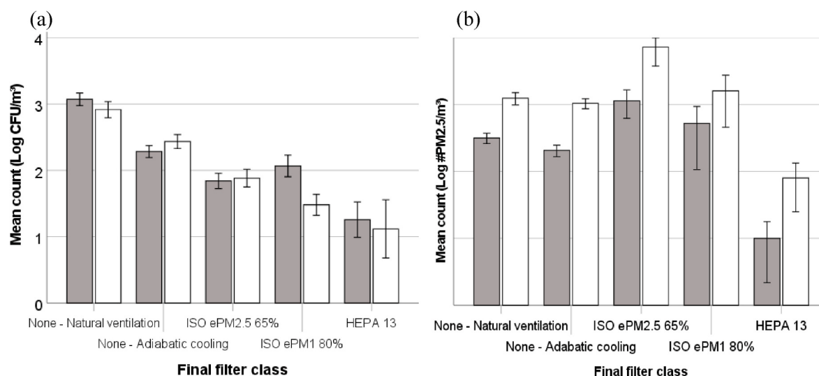
Fig. 7. Influence of final filter class (ISO 16890) on (a) TMPC ■ and Y&M □ and (b) particle size range 1–2.5 µm □ and 2.5–5 µm ■, around the filling area.
