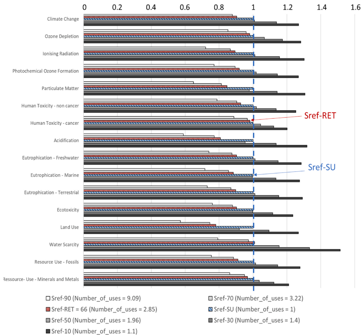
Fig. 5. Life Cycle Impact Assessment of Sref-SU compared to sensitivity scenarios on return rate. For each impact category, the impacts of each sensitivity scenarios are represented in the figure, relatively to Sref-SU, in blue, normalised to 1 for every impact category. The impacts of Sref-RET (corresponding to 66% return rate) are represented in red. The vertical blue bar is the value of Sref-SU for each impact category. Sref-XX is for Sref-RET with return rate = XX%, all other things being equal).
